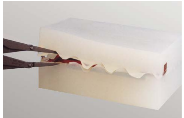
Elastic mould produced by addition curing silicone SikaBiresin® SI291 for optical parts
