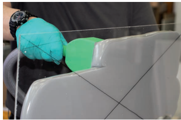
SikaBiresin® SC175 thixotropy enables vertical application in single layer and without sagging
